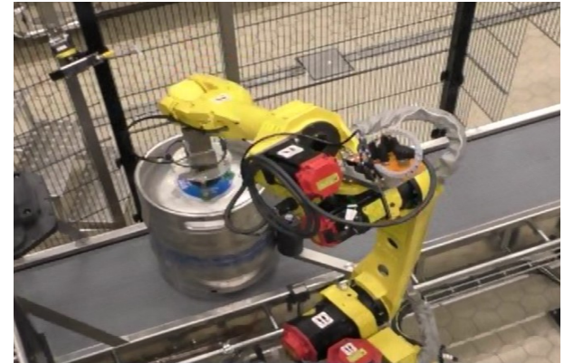
Robot collar & cap applicator
